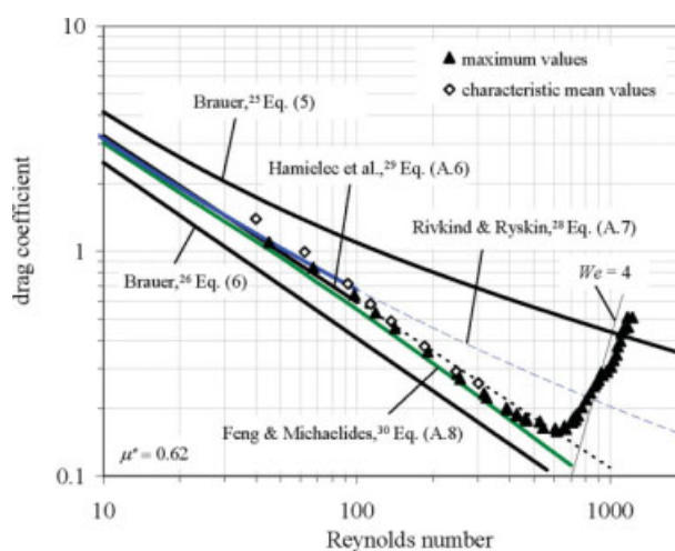
Figure 6. Drag coefficient as a function of Reynolds number.
