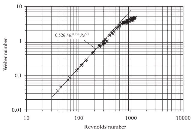
Figure 7. Weber number as a function of Reynolds number.
